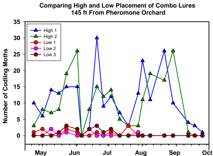
Figure 2. Number of codling moths caught at each date throughout the season comparing combo traps hung high in the top 1/3 of the canopy to traps hung low (~6 ft. from ground) within the pheromone influenced area of the neighboring orchard to the puffer orchard.
