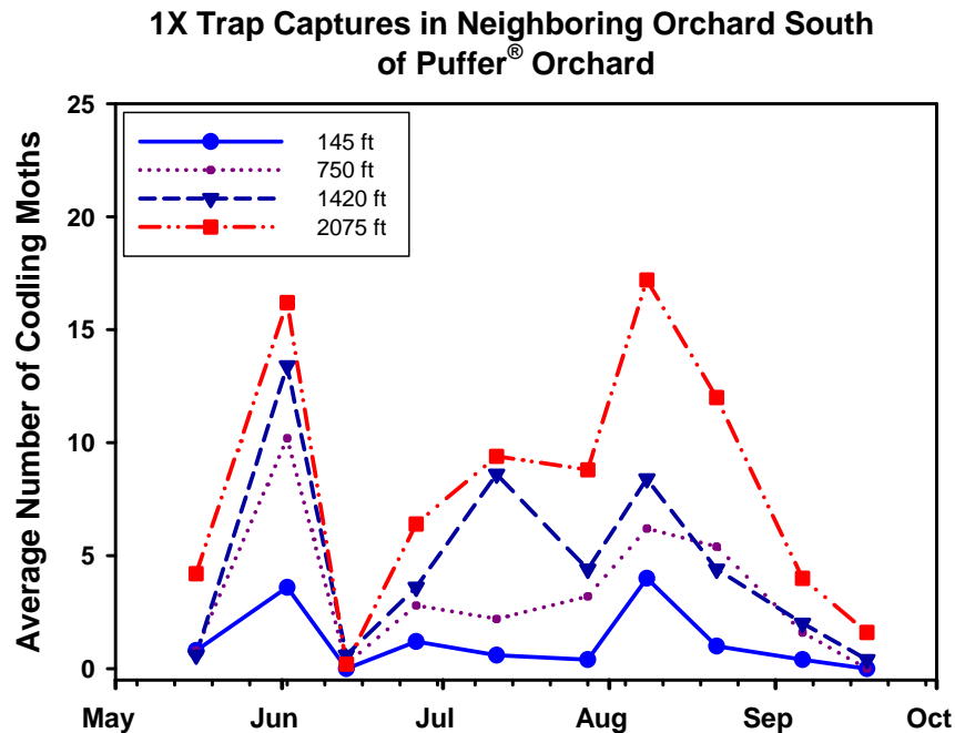
Figure 1. Average codling moth counts over the season in the 1X trap lines at 145, 750, 1,420, and 2,075 feet from puffer orchard.
